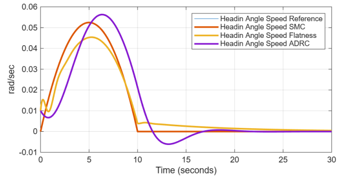
Fig. 4. Heading Angle (rad/sec)
