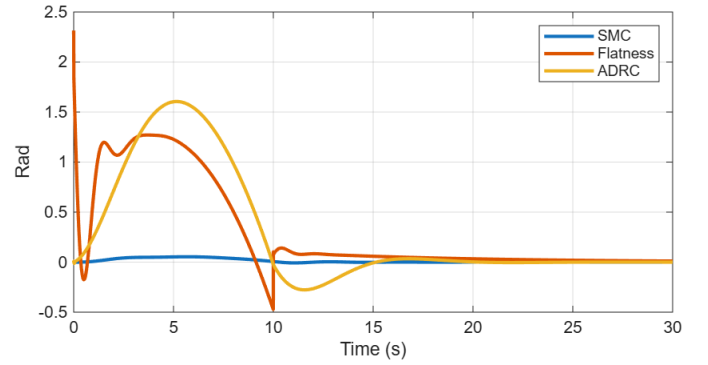
Fig. 2. Steering Angle (rad)
