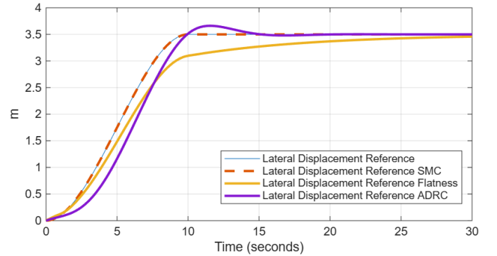
Fig. 3. Lateral Displacement (m)
